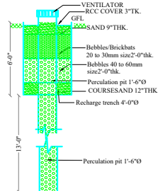
RAIN WATER STORAGE SCALE: 1\"/>
