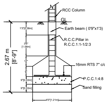
FOUNDATION DETAILS
