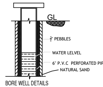
BORE WELL DETAILS
