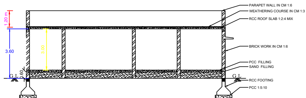
SECTION AB
