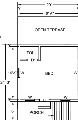
PROPOSED S.F. PLAN
