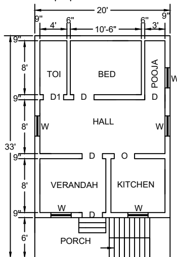
EXISTING F.F. PLAN
