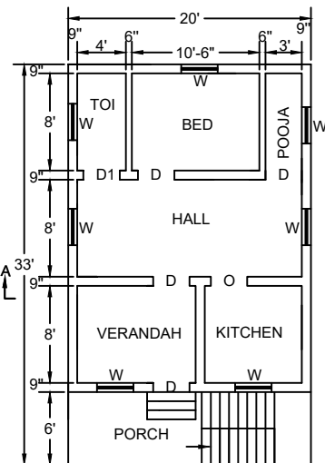
EXISTING G.F. PLAN
