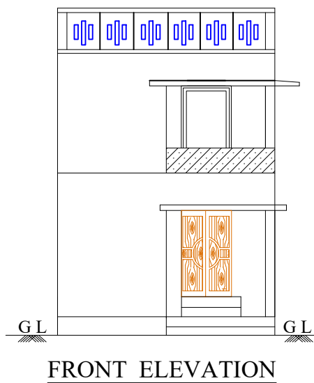
FRONT ELEVATION
