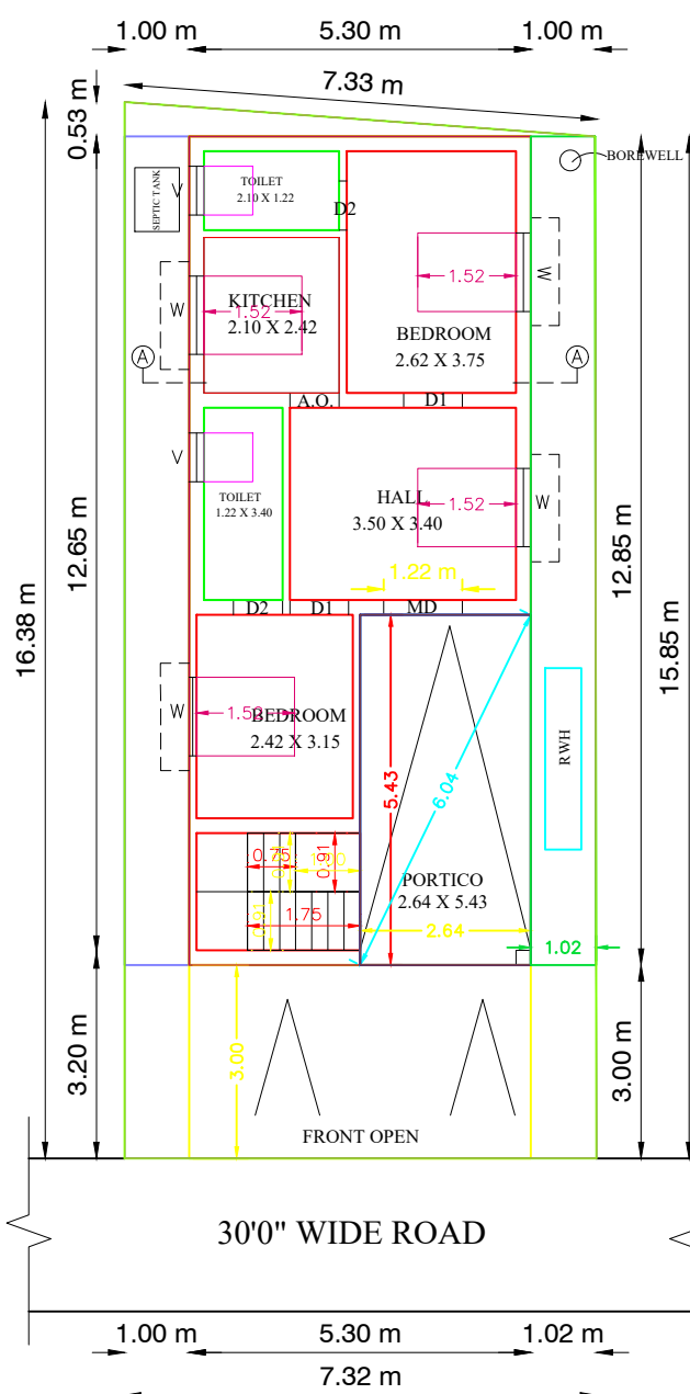
PRO.GROUND FLOOR PLAN
