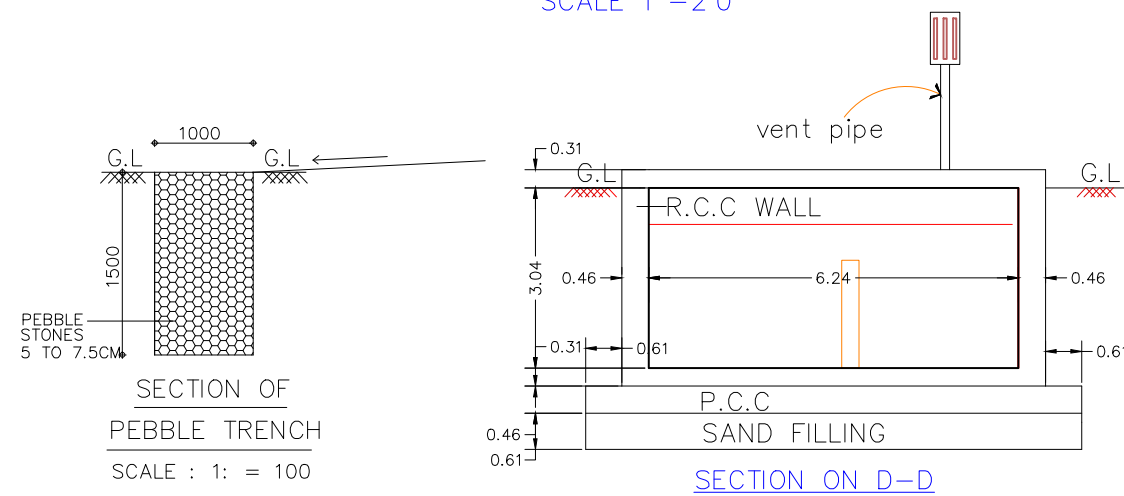
SECTION ON D-D
