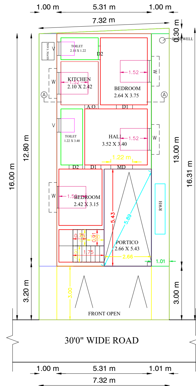
PRO.GROUND FLOOR PLAN
