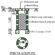
PERCOLATION PIT
