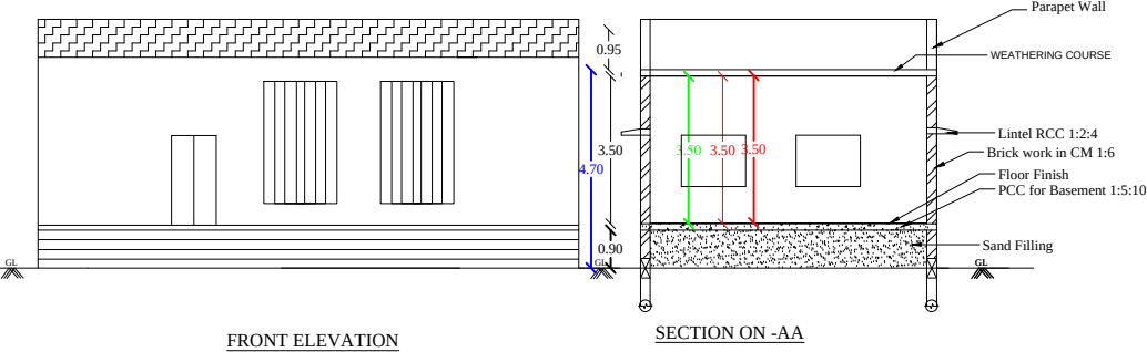
FRONT ELEVATION
