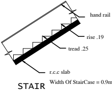
STAIR
