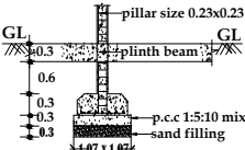
FOUNDATION DETAILS
