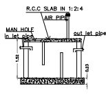
SEPTIC TANK DETAILS
