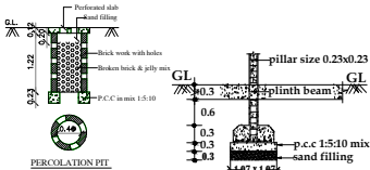
FOUNDATION DETAILS
