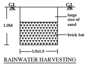
RAINWATER HARVESTING
