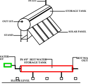
SOLAR HOT WATER SYSTEM DETAILS
