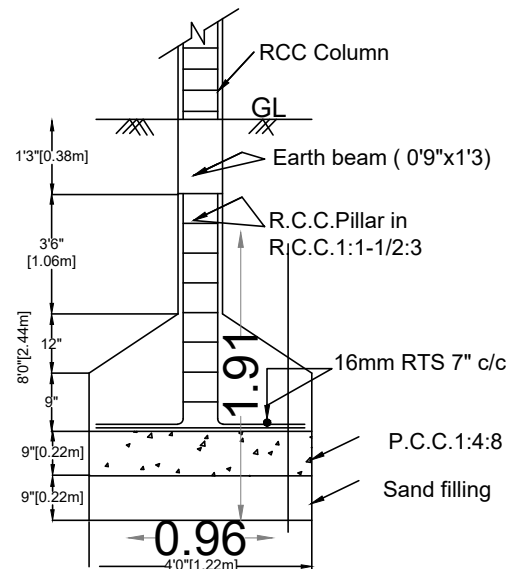
FOUNDATION DETAILS
