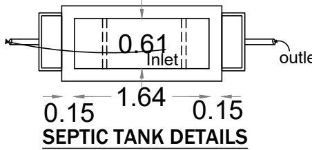
SEPTIC TANK DETAILS
