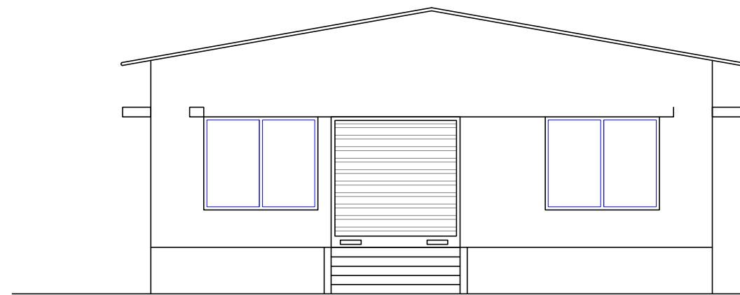
FRONT ELEATION
