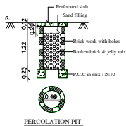
SEPTIC TANK DETAILS
