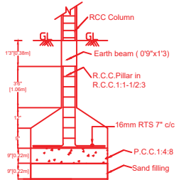
FOUNDATION DETAILS
