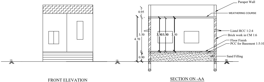
FRONT ELEVATION
