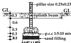
FOUNDATION DETAILS
