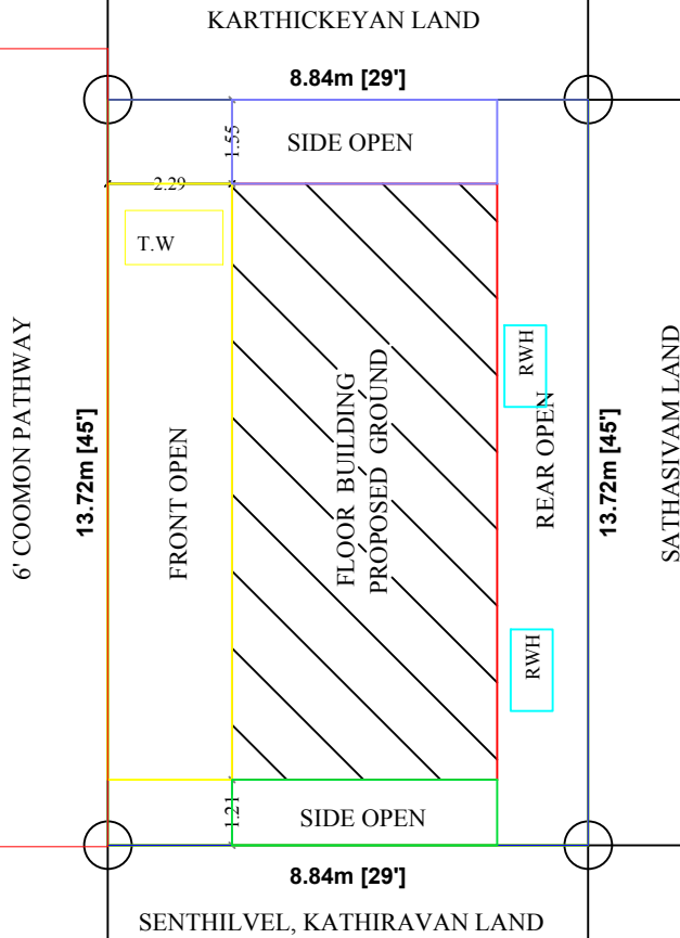
KEY PLAN
