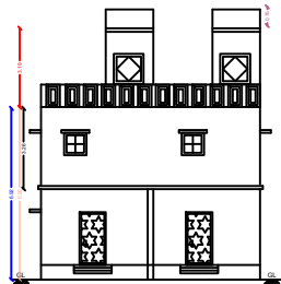
ELEVATION SCALE 1:100
