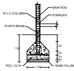
COLUMN DETAILS SCALE 1:100
