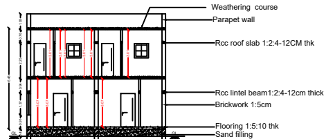
SECTION-AA SCALE 1:100
