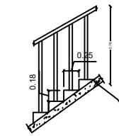
SECTION OF STAIRCASE SCALE 1:100
