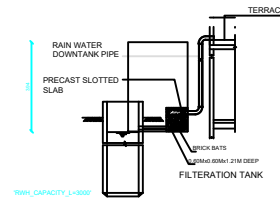
RAIN WATER HARVESTING SYSTEM SCALE 1:100
