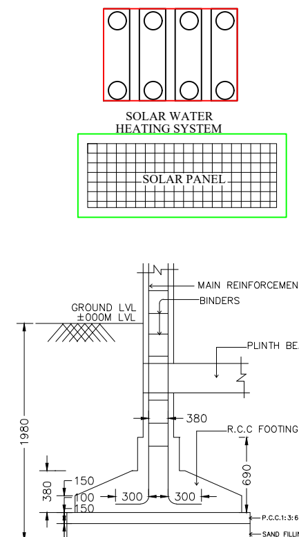
TYPICAL SECTION OF R.C.C. COLUMN FOUNDATION
