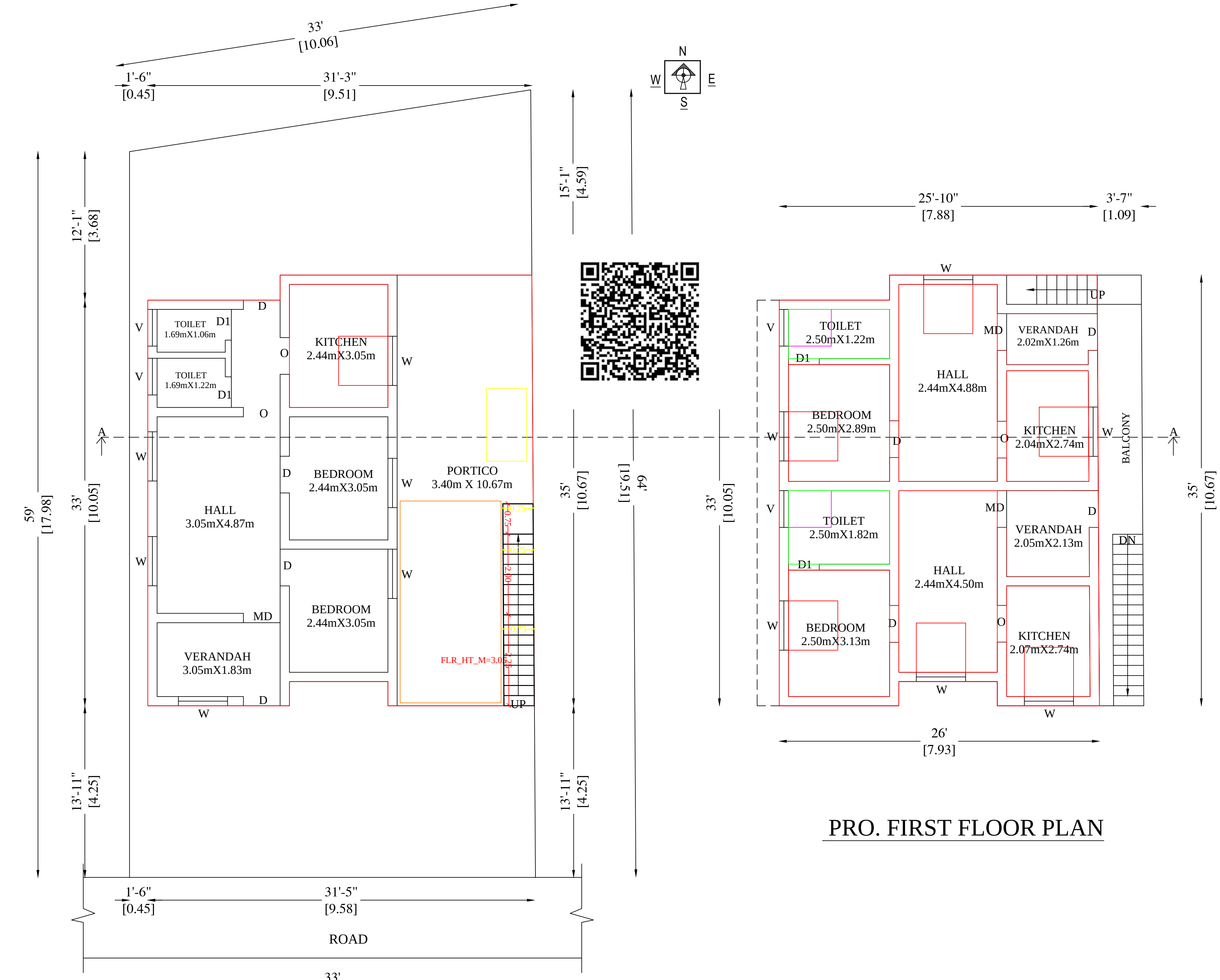
EXG. GROUND FLOOR PLAN
