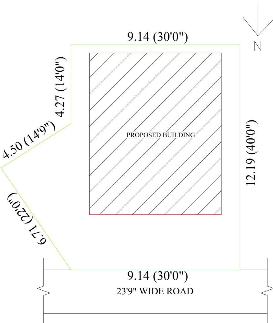
SITE PLAN
