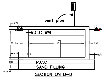
SECTION ON D-D
