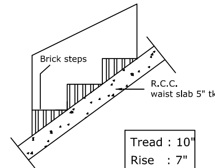
STAIRCASE DETAILS-nts
