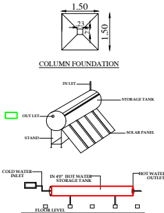
SOLAR HOT WATER SYSTEM DETAILS
