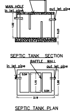
SEPTIC TANK PLAN
