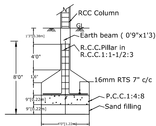
FOUNDATION DETAILS
