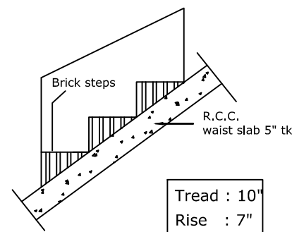
STAIRCASE DETAILS-nts
