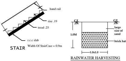
RAINWATER HARVESTING
