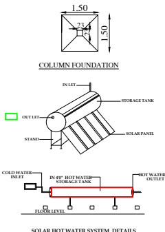
SOLAR HOT WATER SYSTEM DETAILS
