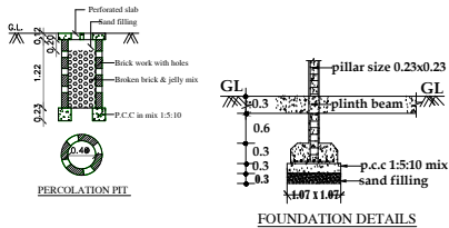
FOUNDATION DETAILS
