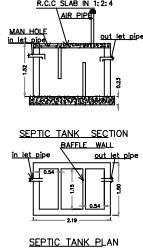
SEPTIC TANK PLAN
