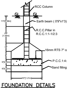
FOUNDATION DETAILS
