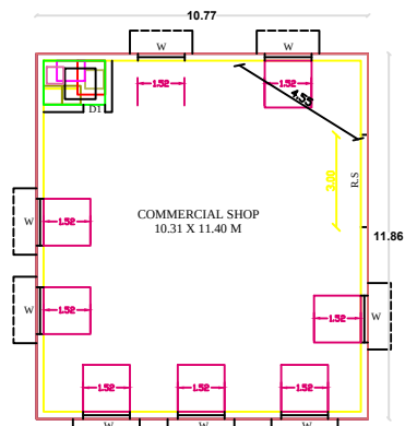
COMMERCIAL GROUND FLOOR PLAN BLOCK II
