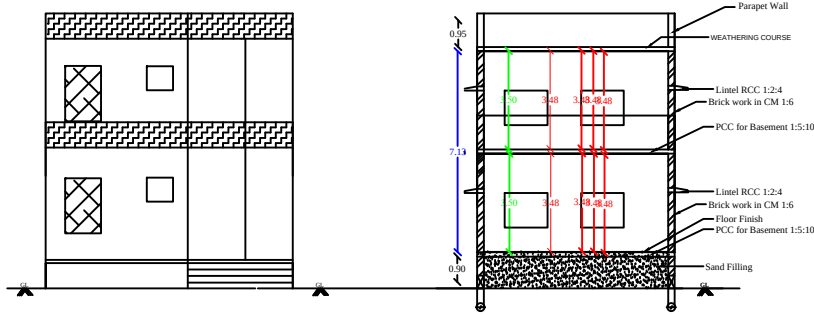
FRONT ELEVATION
