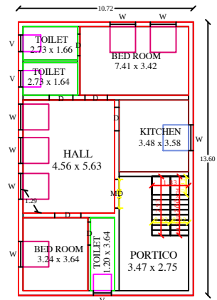
RESIDENTIAL GROUND FLOOR PLAN BLOCK I
