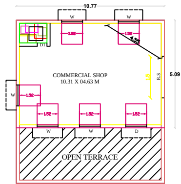
COMMERCIAL FIRST FLOOR PLAN BLOCK II
