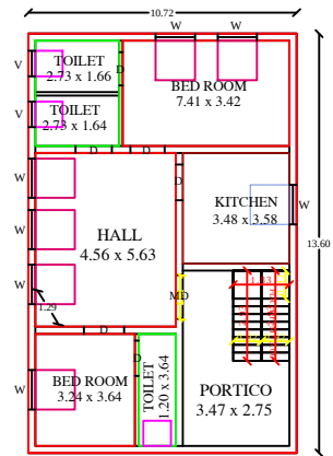
RESIDENTIAL FIRST FLOOR PLAN BLOCK I
