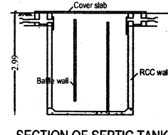
SECTION OF SEPTIC TANK
