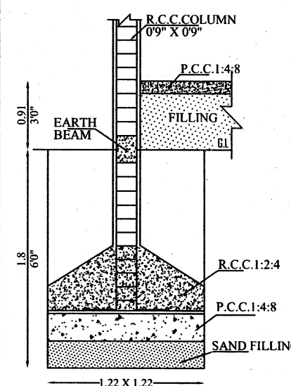
FOUNDATION DETAILS NOT TO SCALE
