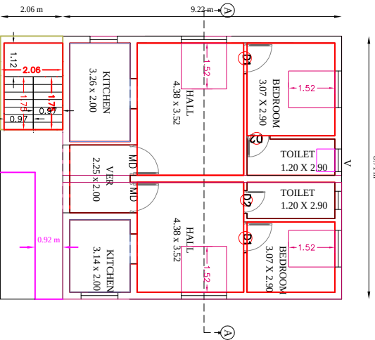
PRO. SECOND FLOOR PLAN
