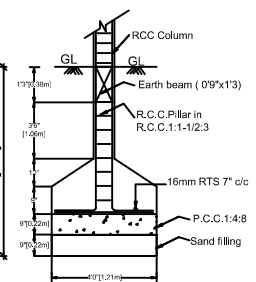
FOUNDATION DETAILS
