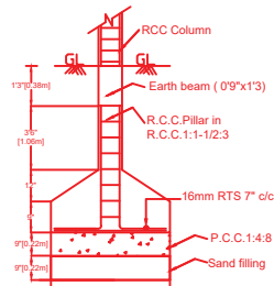
FOUNDATION DETAILS
