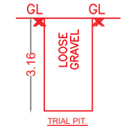
TRIAL PIT
