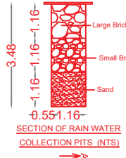
SECTION OF RAIN WATER COLLECTION PITS (INTS)
