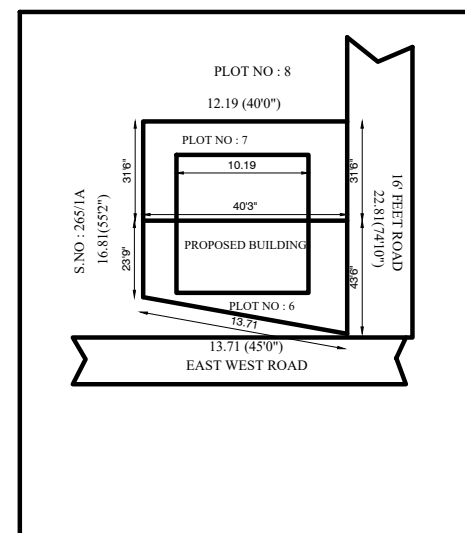
SITE PLAN(NTS)
