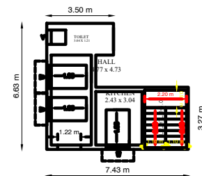
PROPOSED SECOND FLOOR PLAN
