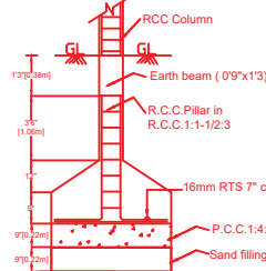
FOUNDATION DETAILS
