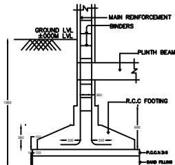
TYPICAL SECTION OF R.C.C. COLUMN FOUNDATION SCALE : 1" = 2'-0"
