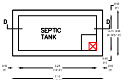
PLAN OF SEPTIC TANK SCALE 1"=2'0"
