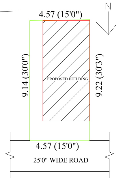
SITE PLAN
