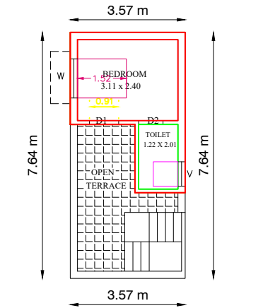
PRO.FIRST FLOOR PLAN
