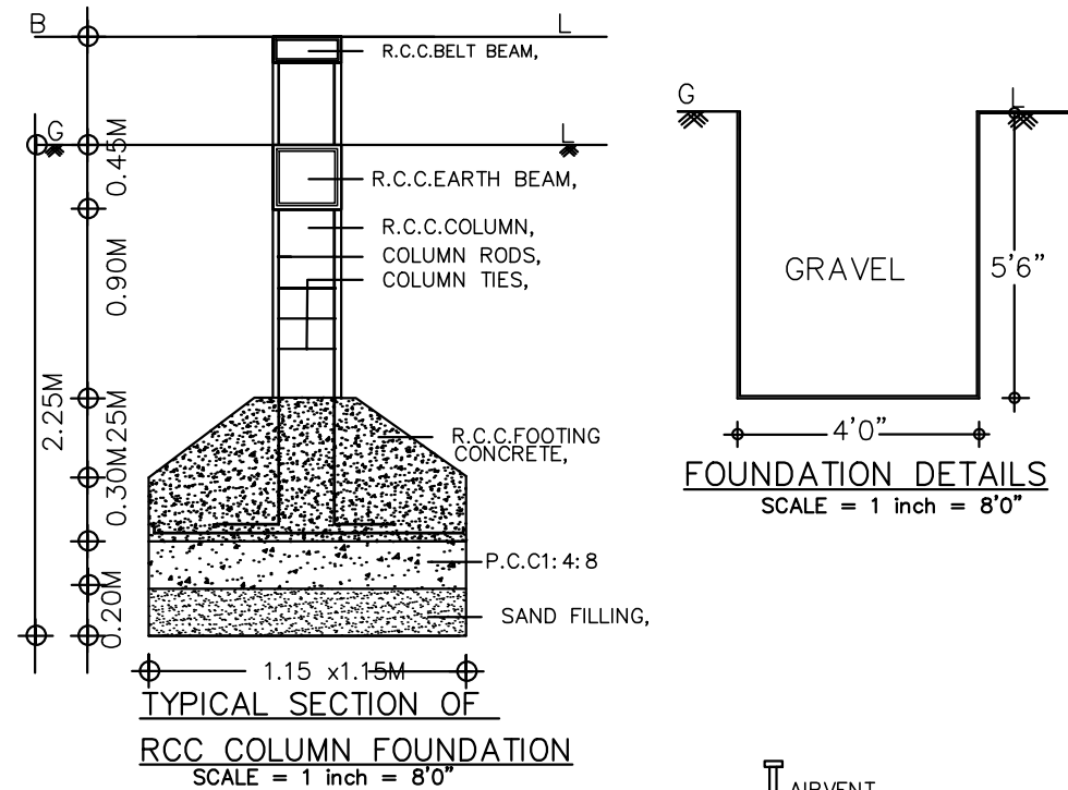
TYPICAL SECTION OF RCC COLUMN FOUNDATION
