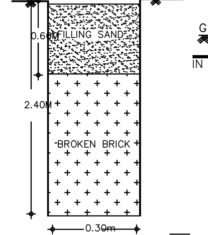
RAIN WATER HARVEST PIT SCALE = 1 inch = 8'0"
