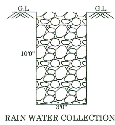
RAIN WATER COLLECTION PIT
