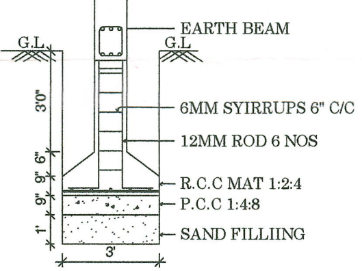
FOOTING DETAILS
