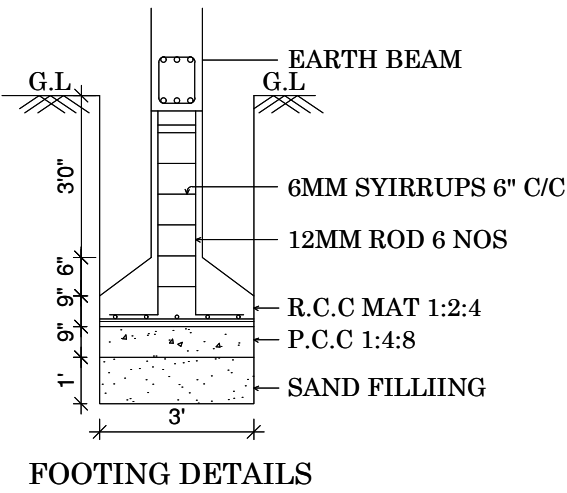
FOOTING DETAILS
