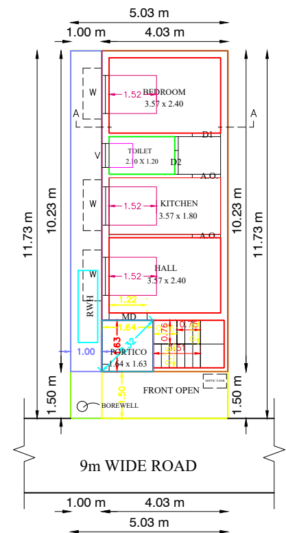
PRO.GROUND FLOOR PLAN
