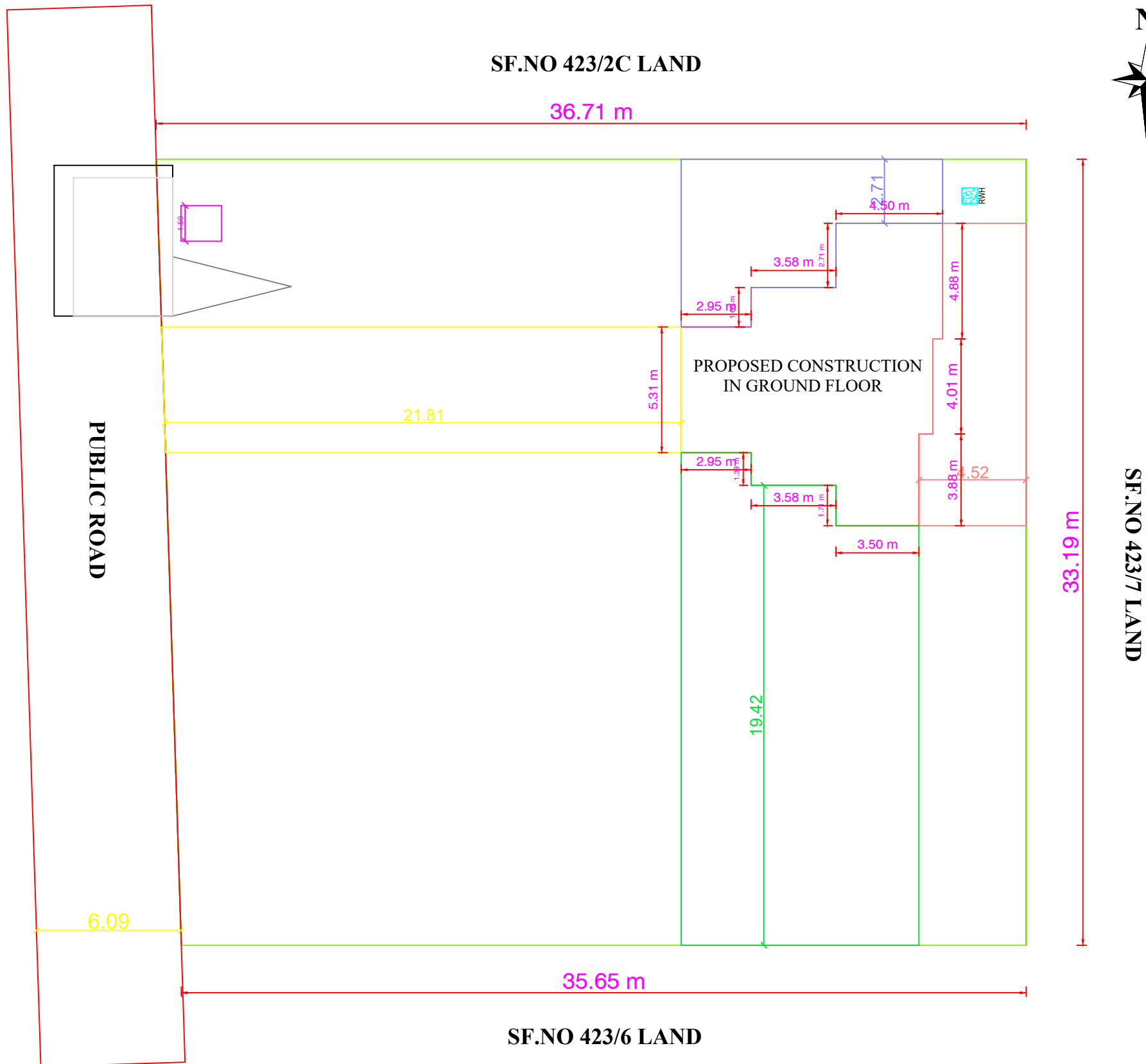
SITE PLAN
