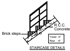
STAIRCASE DETAILS
