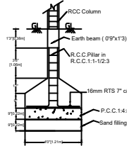
FOUNDATION DETAILS
