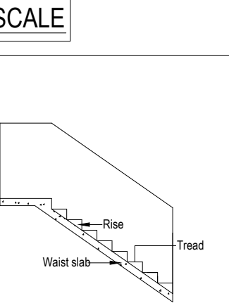
DETAILS OF STAIR CASE
