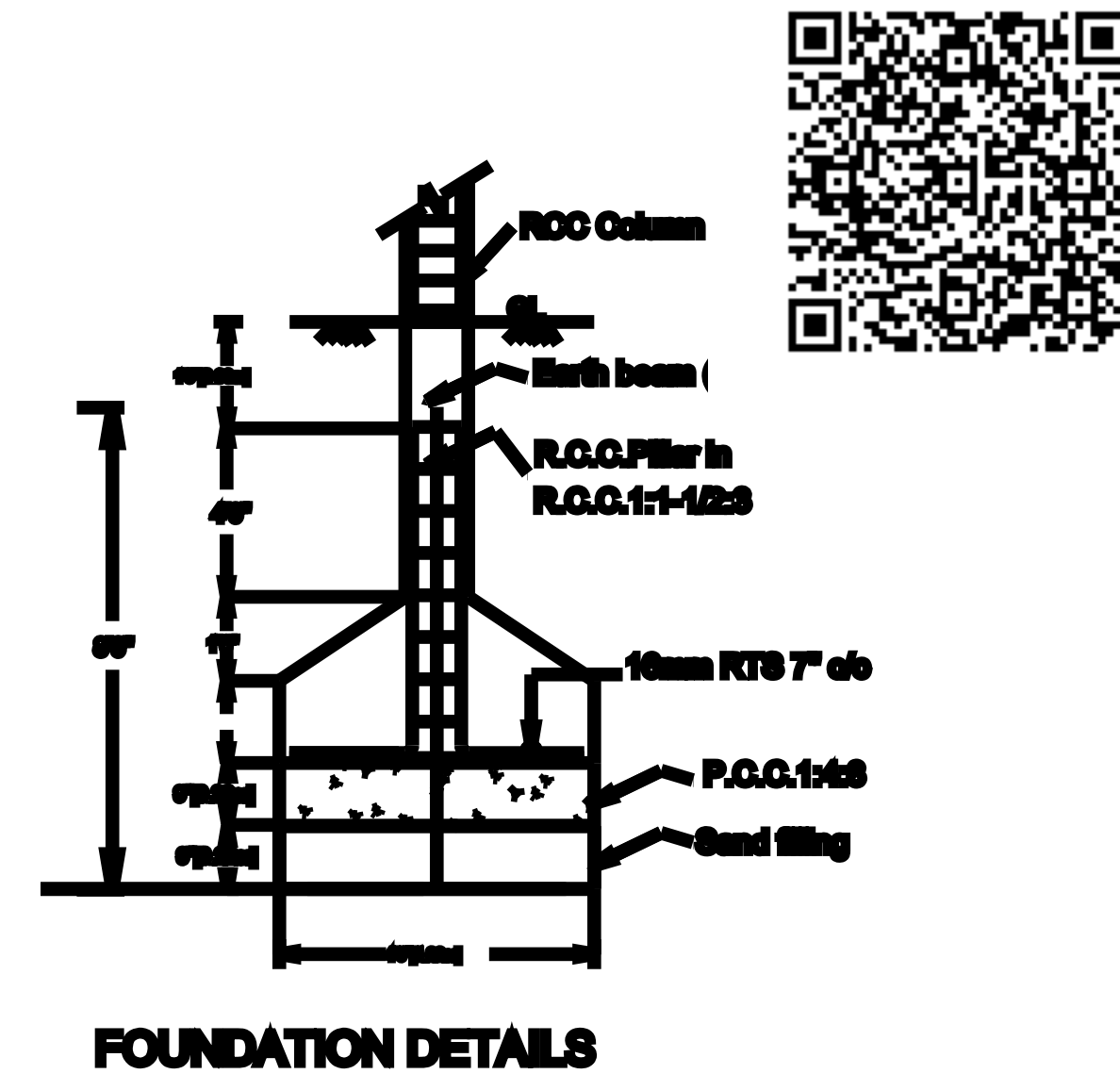
FOUNDATION DETAILS
