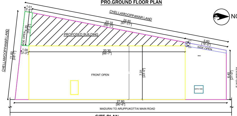
SITE PLAN
