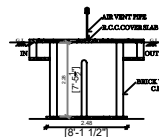
SEPTIC TANK DETAILS-SECTION
