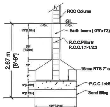
FOUNDATION DETAILS
