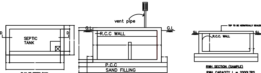
PLAN OF SEPTIC TANK SCALE 1"=2'0"
