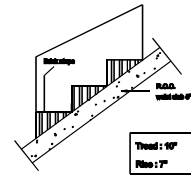
STAIRCASE DETAILS-cls
