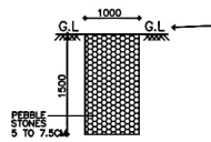
SECTION OF PEBBLE TRENCH SCALE : 1: = 100
