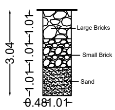
SECTION OF RAIN WATER COLLECTION PITS (NTS)
