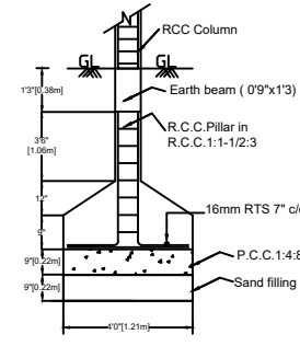
FOUNDATION DETAILS
