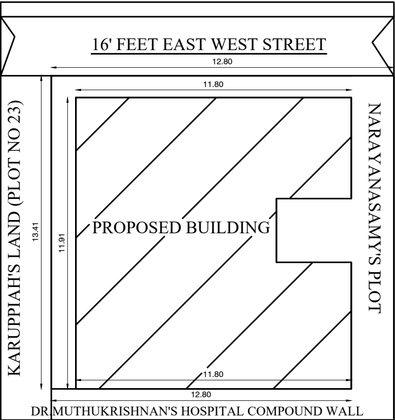
SITE PLAN
